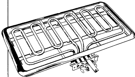
Cat No. 2490 2400 Watt Grill Boiler Suits - Everhot/Malleys Email - 1019G1
