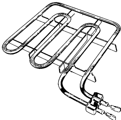
Cat No. 1782LH (left hand) 1200 Watt Grill Boiler Suits Malleys, GEC/BGE Email GH700 Socket 1782-20
