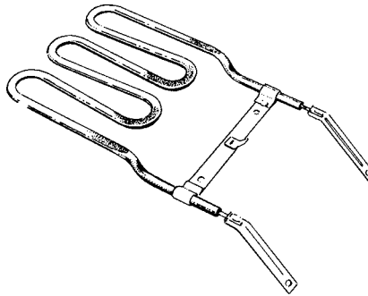
Cat No. 293-23 850 Watt Grill Suits - Vulcan Email - 91324G1
