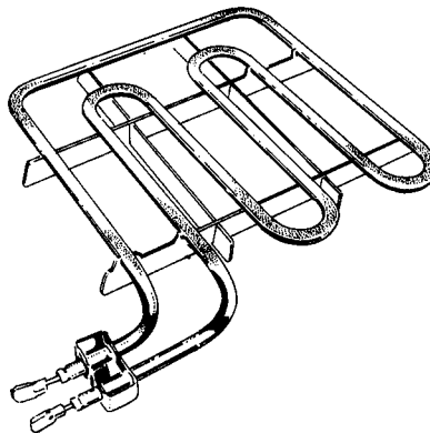
Cat No. 1783RH (right hand) 1200 Watt Grill Boiler Suits Malleys, GEC/BGE Email GH701 Socket 1782-20
